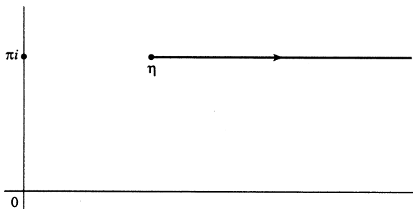
FIGURE 8.1 Integration Contour
